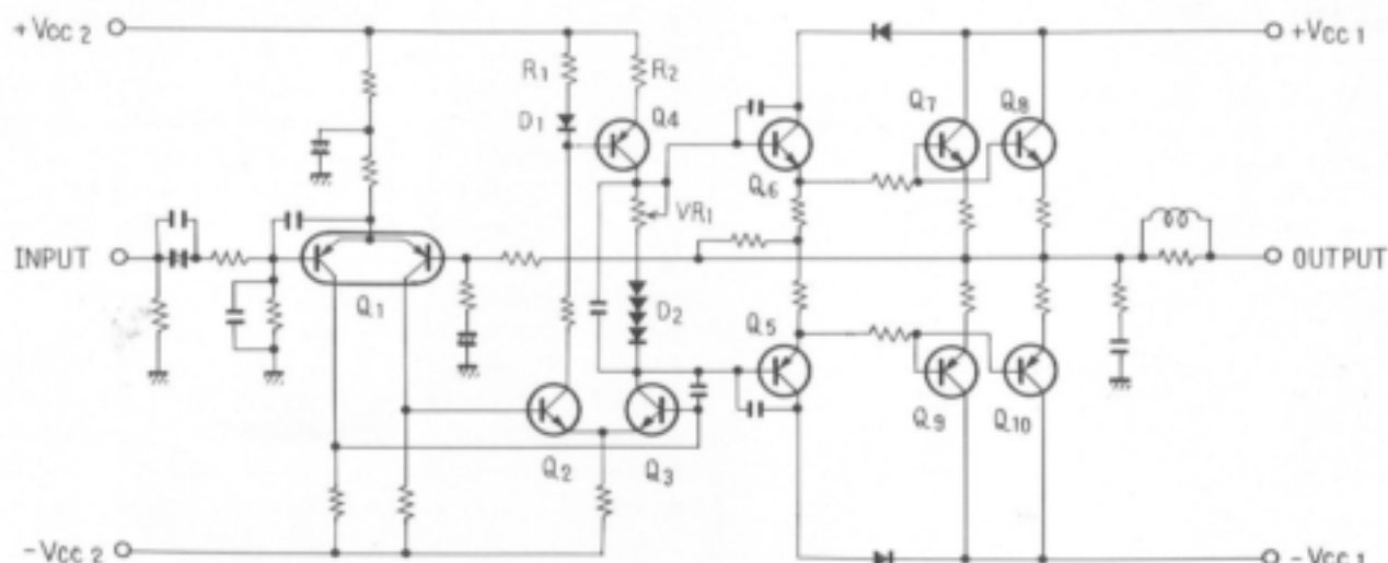
Fig. 6. Schematic diagram for power amplifier
